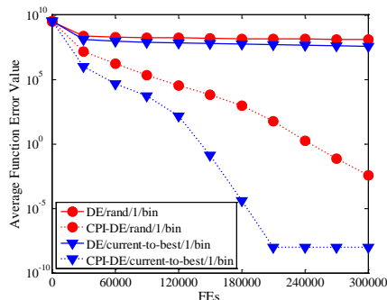
(a) CEC2013 2 with 30D
