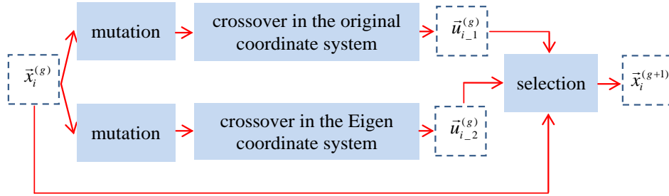
Fig. 2. The mutation, crossover, and selection of CPI-DE.
