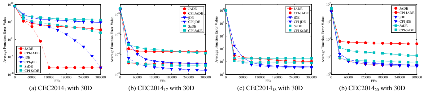
Fig. 5. Evolution of the average function error values derived from three state-of-the-art DE variants (JADE, jDE, and SaDE) and their augmented algorithms versus the number of FEs on CEC2014 1 with 30D, CEC2014 17 with 30D, CEC2014 18 with 30D, and CEC2014 20 with 30D
