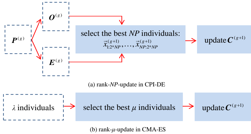
Fig. 3. The relationship between rank- NP -update in CPI-DE and rank- \mu -update in CMA-ES.
