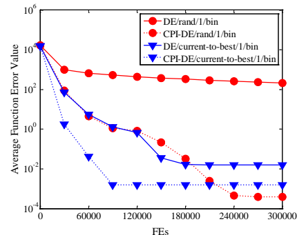
(b) CEC2013 10 with 30D
