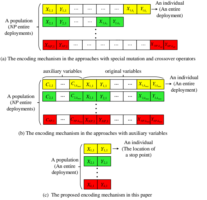
Fig. 2. Encoding mechanism in the approaches with special mutation and crossover operators, encoding mechanism in the approaches with auxiliary variables, and the proposed encoding mechanism in this paper, where X_{i,j} and Y_{i,j} denote the values in the x -axis and y -axis of the location of the j th stop point in the i th individual, respectively; C_{i,j} denotes the j th auxiliary variable in the i th individual; and k_{max} is the maximum number of stop points as defined in (14).
