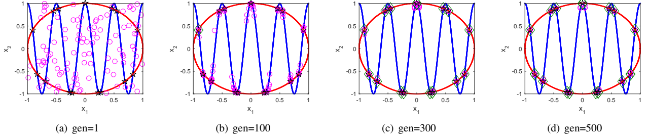
Fig. 6. Evolution of RADE over a typical run on F03. Circles denote the individuals in the population, pentagrams denote the known roots, and diamonds denote the found roots in the archive.
