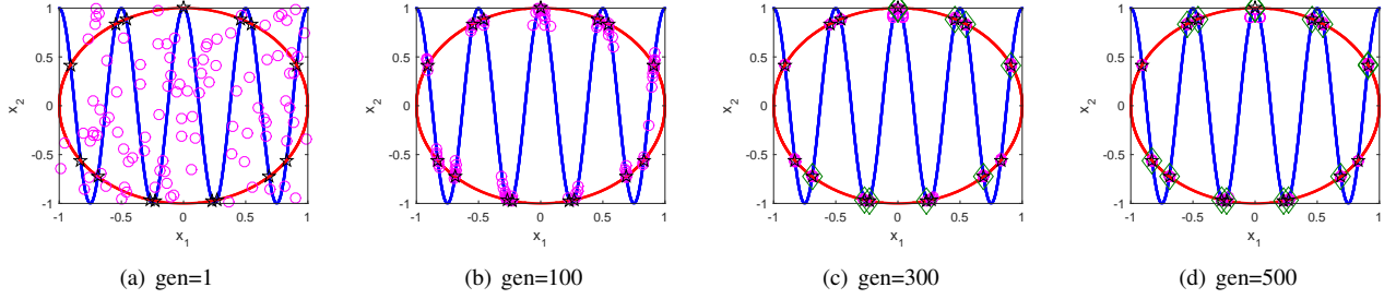
Fig. 5. Evolution of RADE-WoA over a typical run on F03. Circles denote the individuals in the population, pentagrams denote the known roots, and diamonds denote the found roots in the archive.
