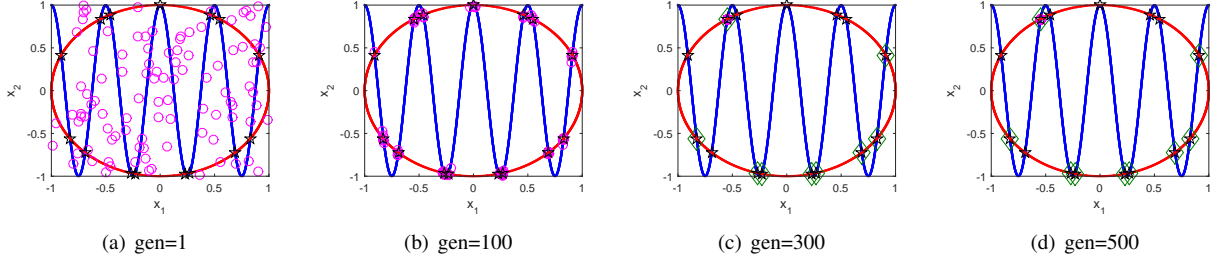
Fig. 4. Evolution of RADE-WoD over a typical run on F03. Circles denote the individuals in the population, pentagrams denote the known roots, and diamonds denote the found roots in the archive.
