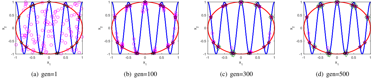
Fig. 3. Evolution of RADE-WoR over a typical run on F03. Circles denote the individuals in the population, pentagrams denote the known roots, and diamonds denote the found roots in the archive.
